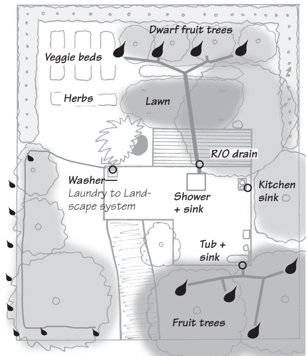
SAMPLE GREYWATER DISTRIBUTION PLAN WITH LAUNDRY TO LANDSCAPE AND GRAVITY-FLOW BRANCHED DRAIN SYSTEMS
