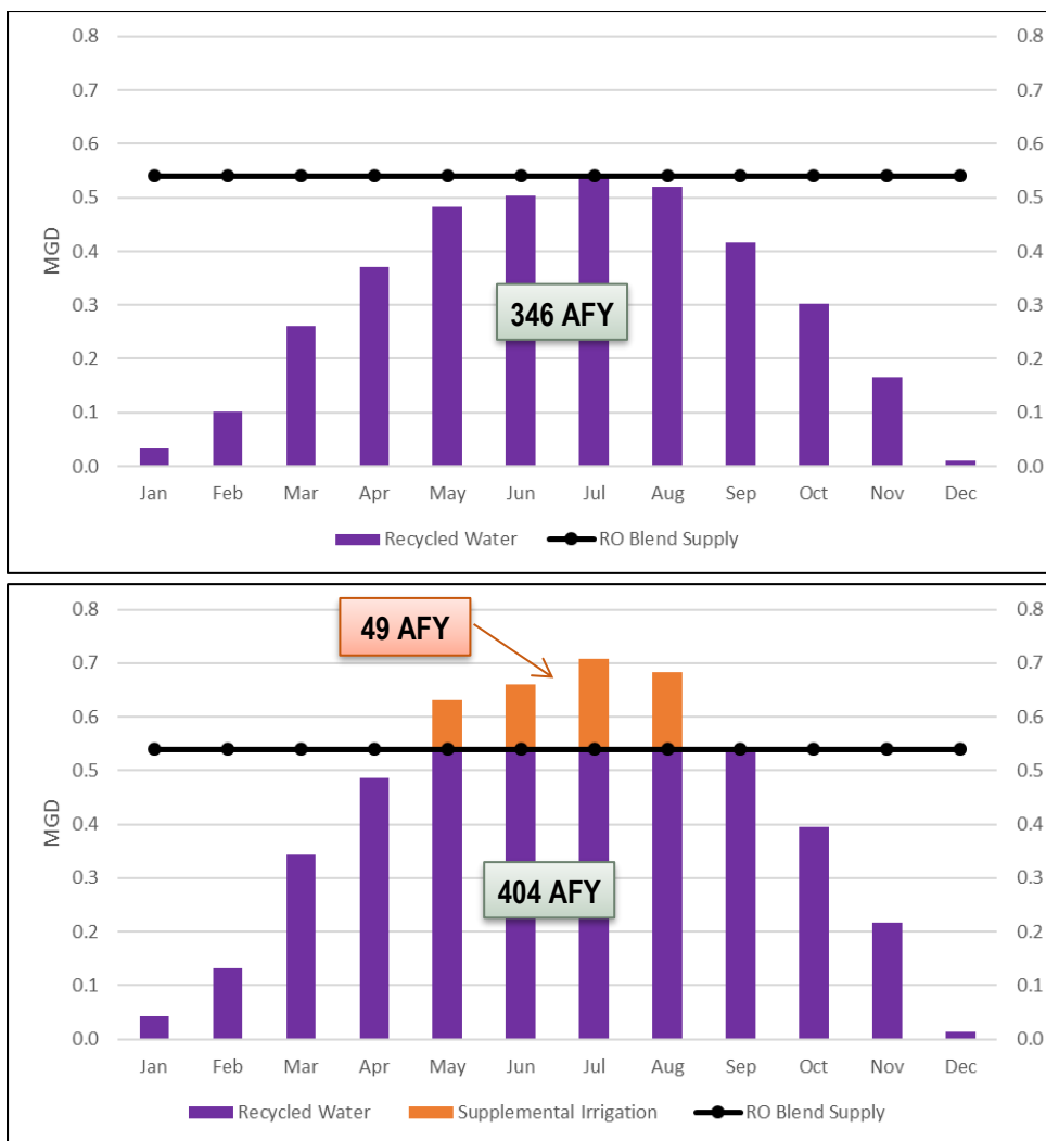
Figure 17: Example Monthly Seasonal Irrigation Demand
