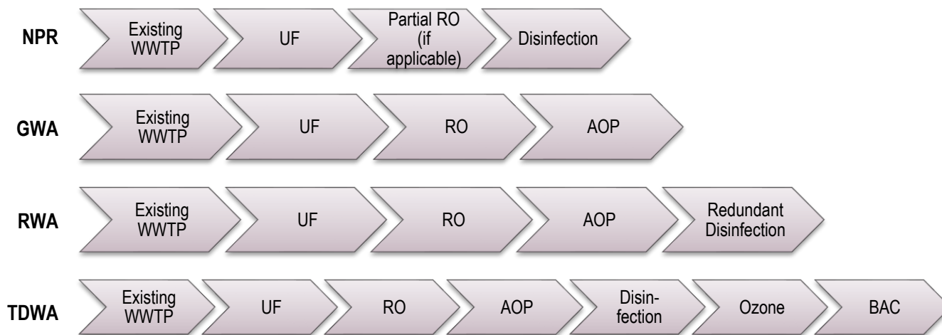
Figure 15: Recycled Water Treatment Requirement Assumptions
