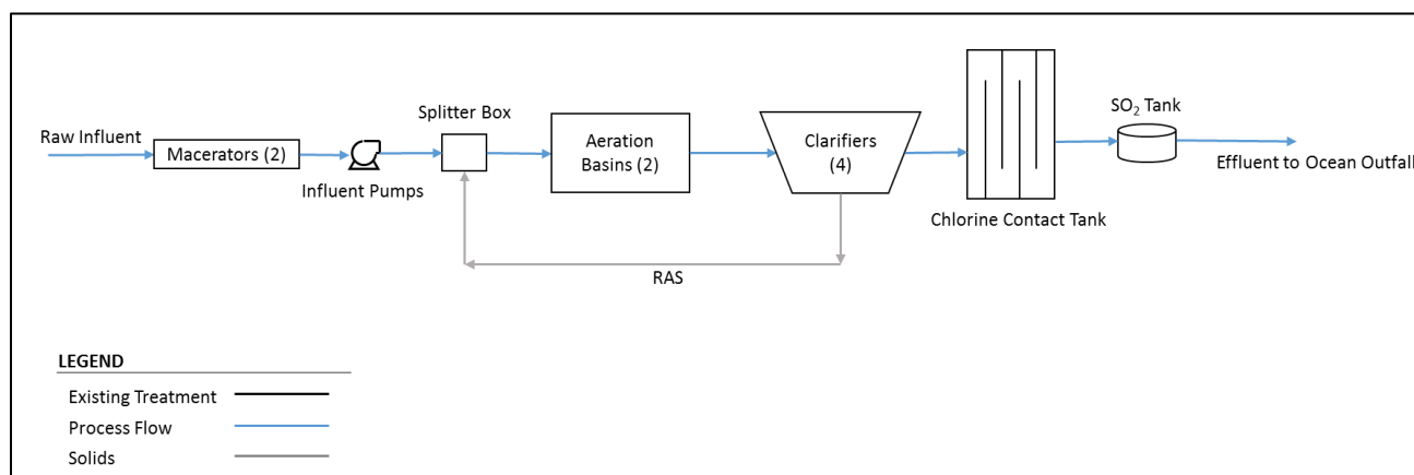
Figure 7: Montecito WWTP Flow Schematic
