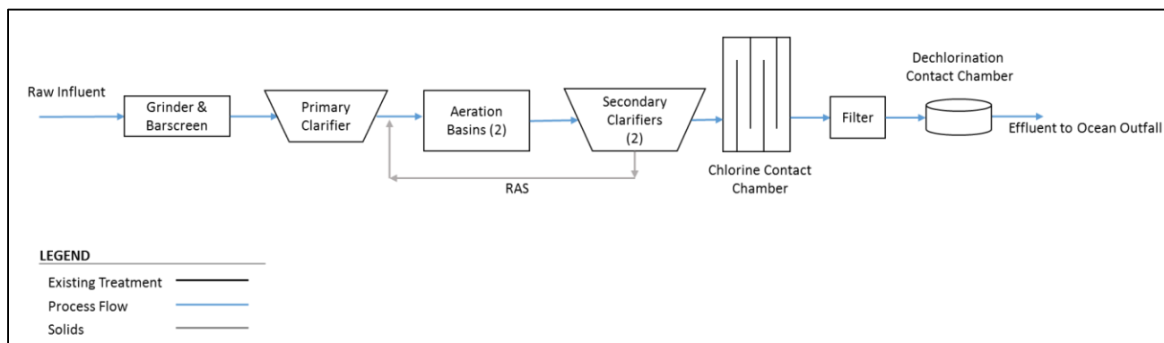
Figure 9: Summerland WWTP Flow Schematic
